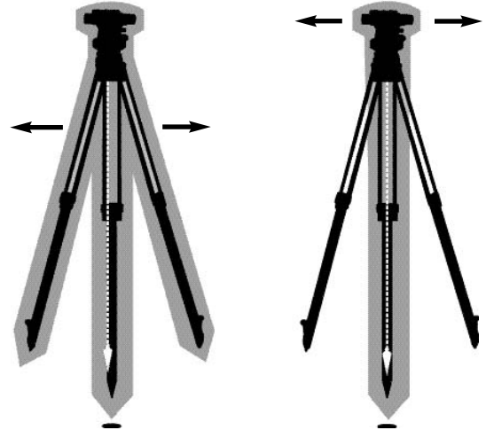
1. Move tripod and instrument over the approximate point
