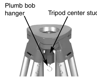
\frac{3}{8} X 11 tribrach tripod
